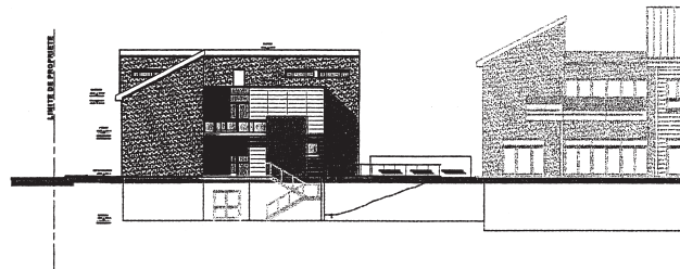
FACADE ARRIERE
