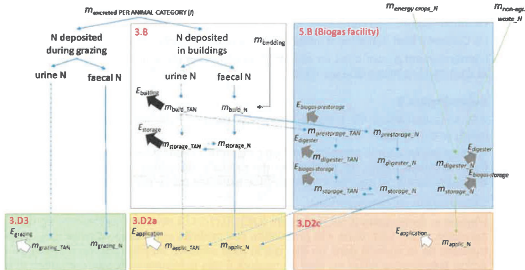
Figure 5-6 – N flow in the manure management system
